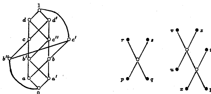
Figure 7. A poset with its monotone zigzags
