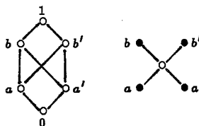
Figure 1. Poset P and a P-zigzag (H, f)
