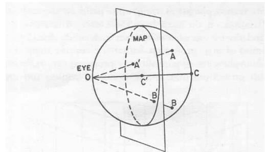
Figure 31. The principle of the stereographic projection
