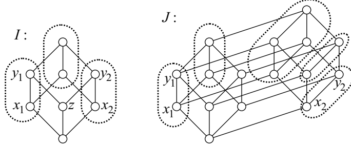
FIGURE 1. Two ideals in B_m
