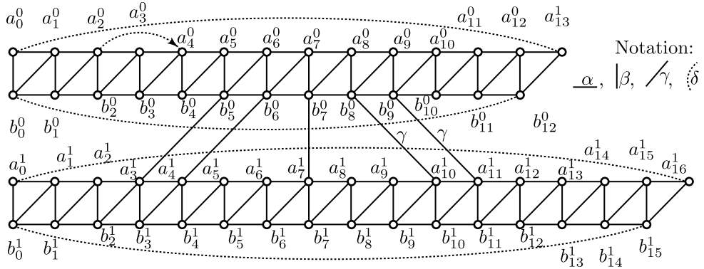
FIGURE 2. F_{13} \oplus F_{16}
