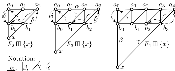
FIGURE 3. F_n \boxplus \{x\} for n \in \{2, 3, 4\}
