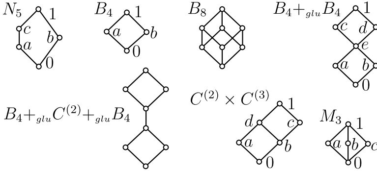
FIGURE 2. Lattices for Theorem 1 and Lemma 2
