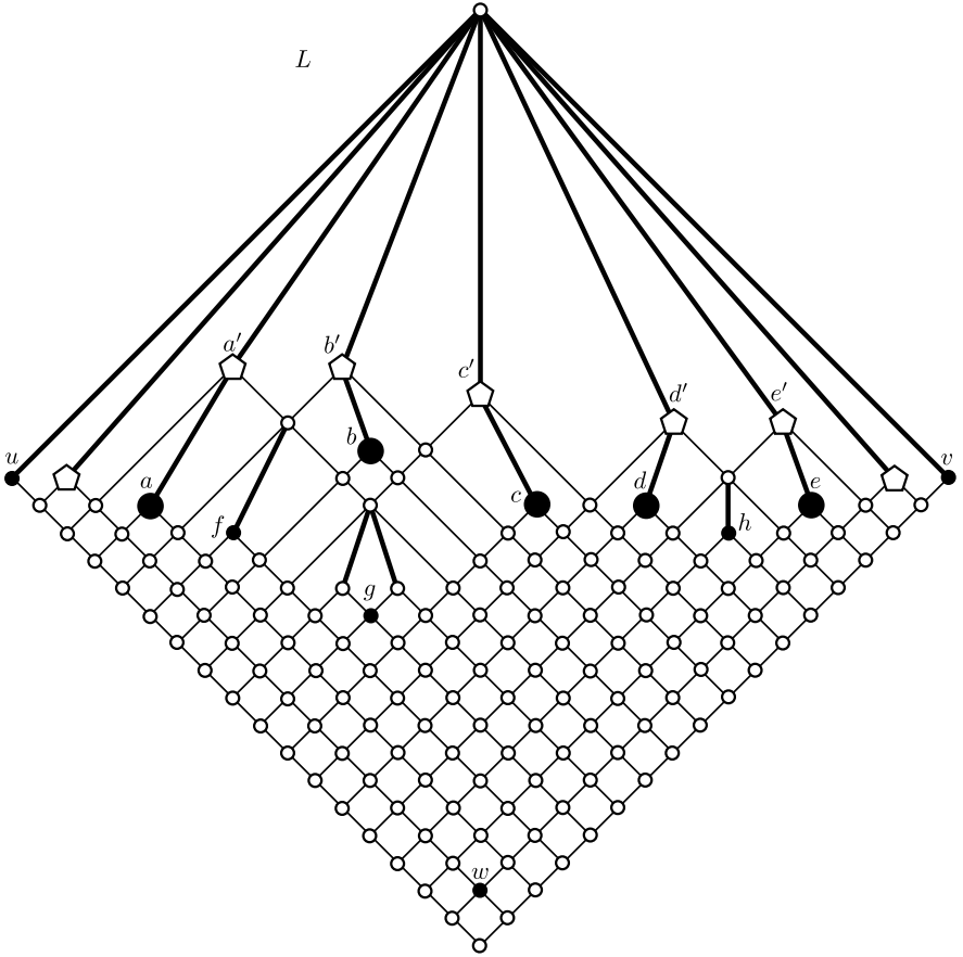
FIGURE 12. A C_2 -diagram of L
