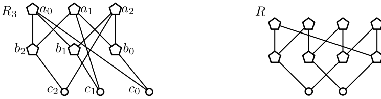
FIGURE 1. The Three-pendant Three-crown ordered set R_3 and the Two-pendant Four-crown ordered set R ; the elements of the crowns are indicated by pentagons
