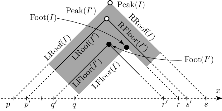
FIGURE 5. Case p < p' < q
