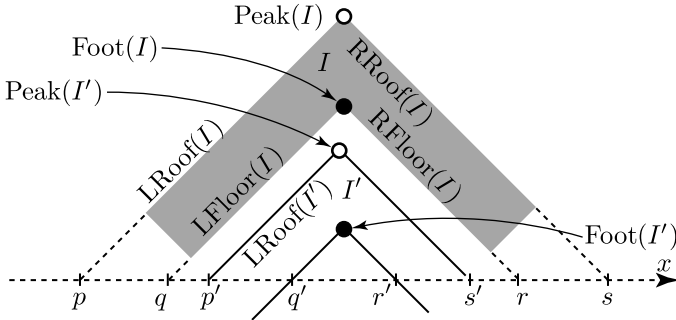
FIGURE 6. Case p < p' and s' < s
