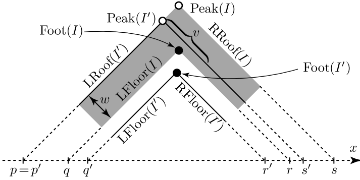
FIGURE 3. Proving (4.10)
