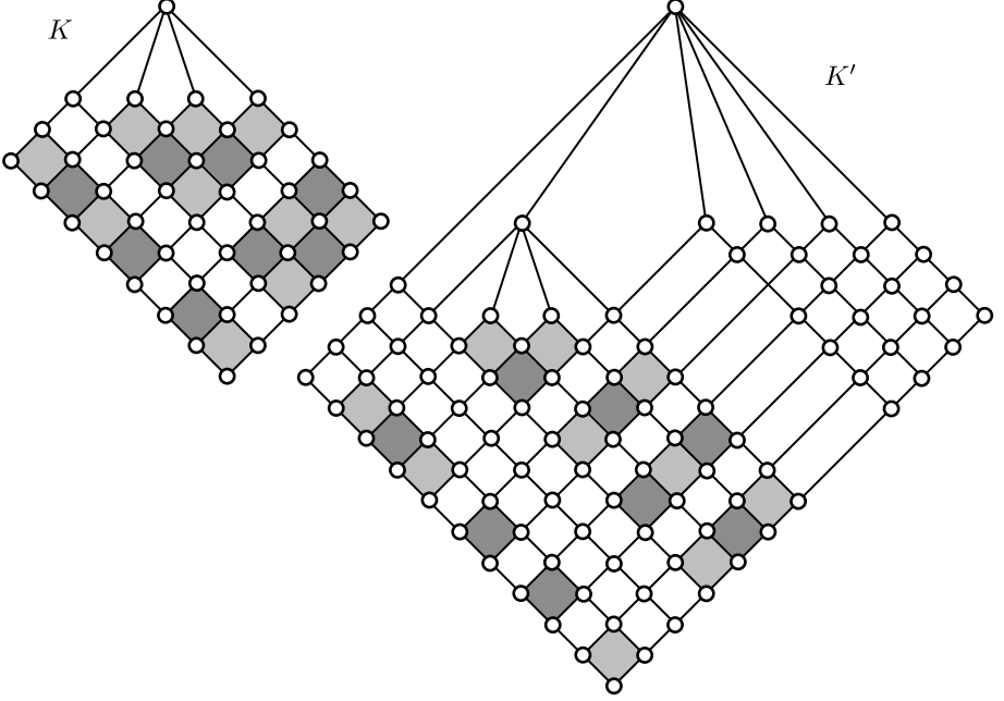
FIGURE 10. Illustrating Lemma 6.2
