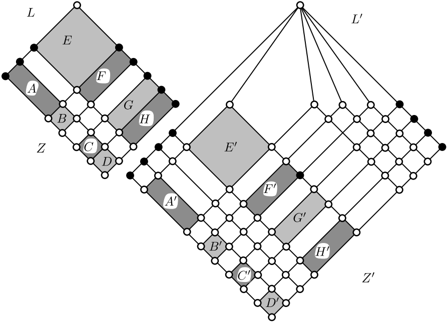
FIGURE 9. Z and Z' have the same distance-free geometry
