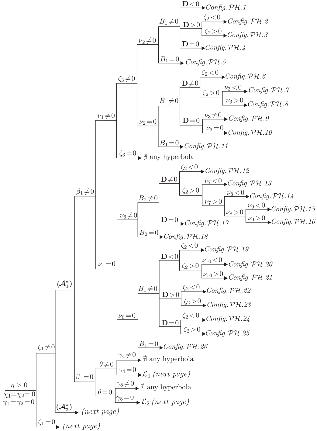
Diagram 1.1: Conditions for configurations for systems in QSPH: the case \eta > 0
