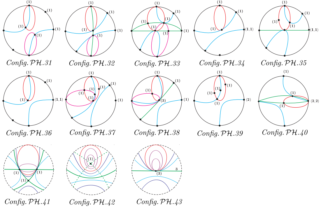
Figure 1.1 (cont.) Configurations of quadratic systems in QSPH
