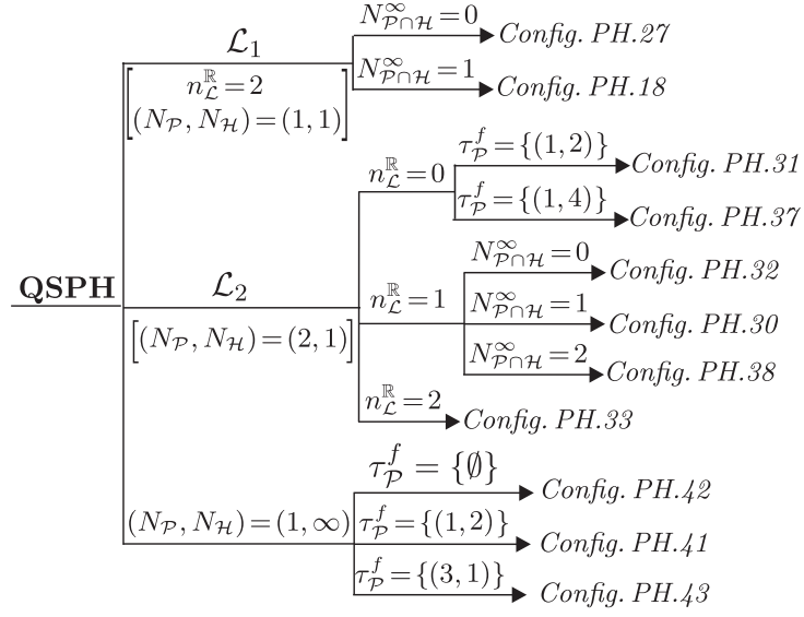
Diagram 3.1 (contin.) Non-equivalent configurations of systems in QSPH
