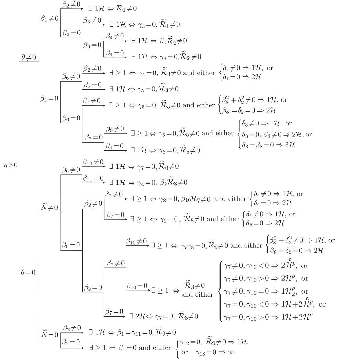
Diagram 2.1: Existence of invariant hyperbolas: the case \eta > 0
