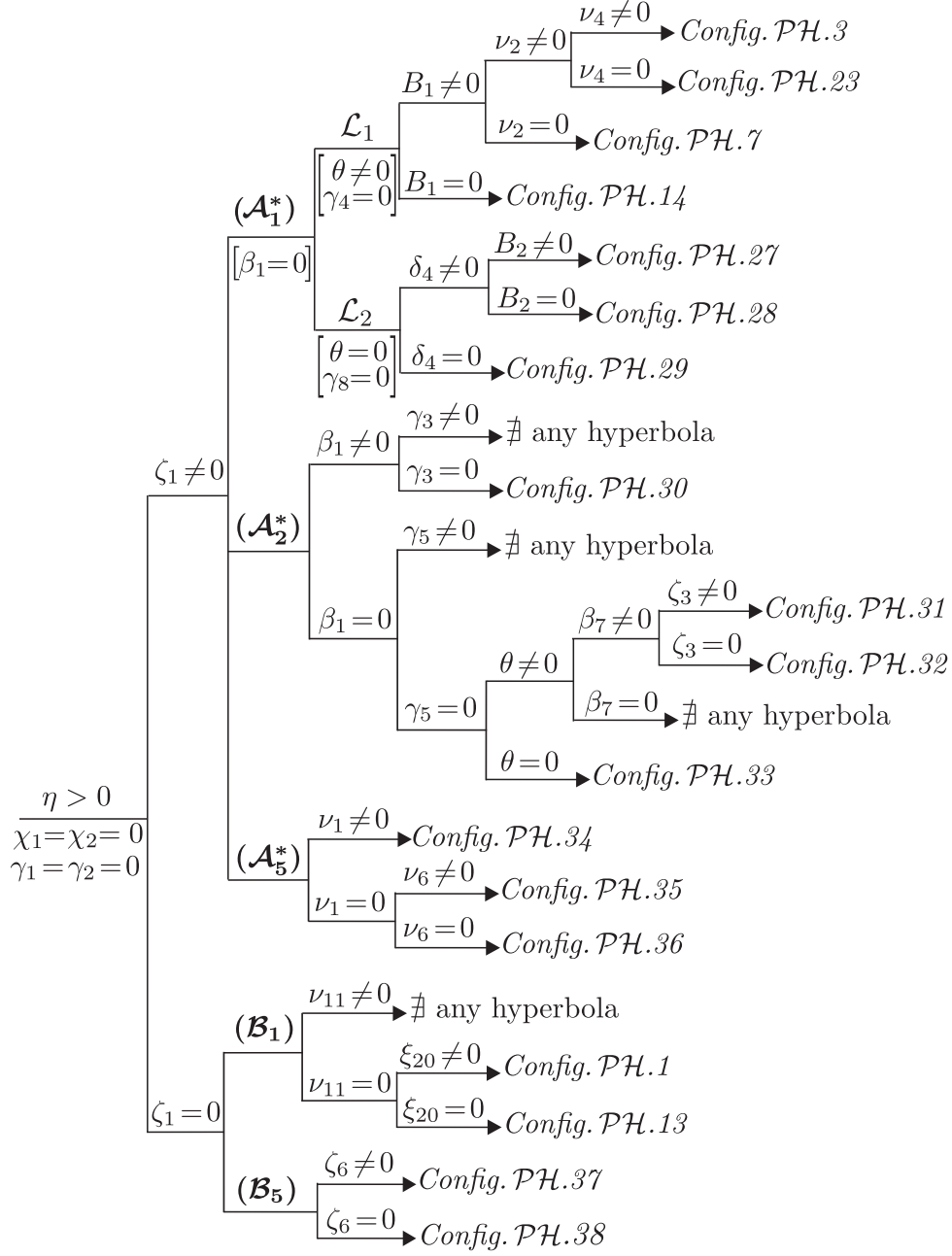
Diagram 1.1 (cont.) Conditions for configurations for systems in QSPH : the case \eta > 0
