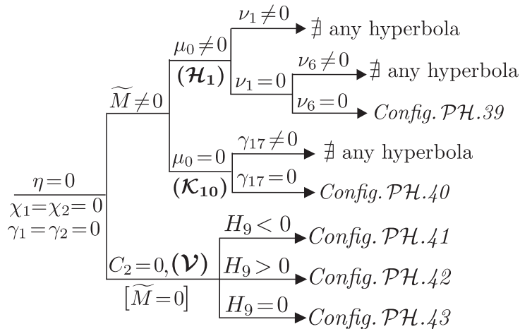
Diagram 1.2: Conditions for configurations for systems in QSPH : the case \eta = 0
