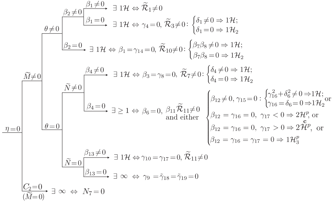
Diagram 2.2: Existence of invariant hyperbolas: the case \eta = 0
