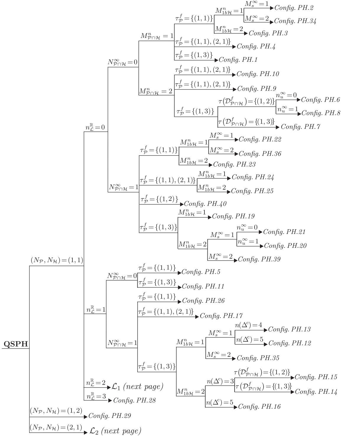
Diagram 3.1: Non-equivalent configurations of systems in QSPH
