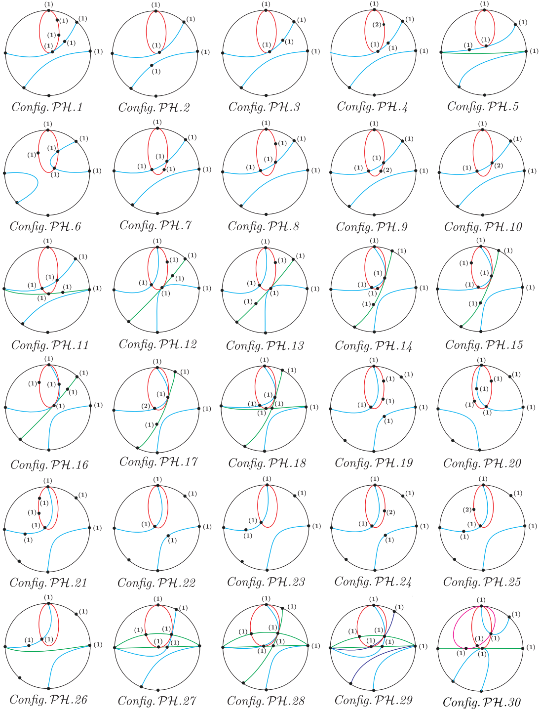
Figure 1.1: Configurations of quadratic systems in QSPH
