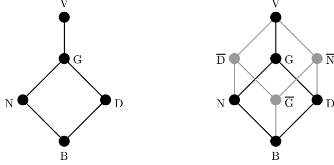
Fig. 1. The lattice Y and its embedding into a power set
