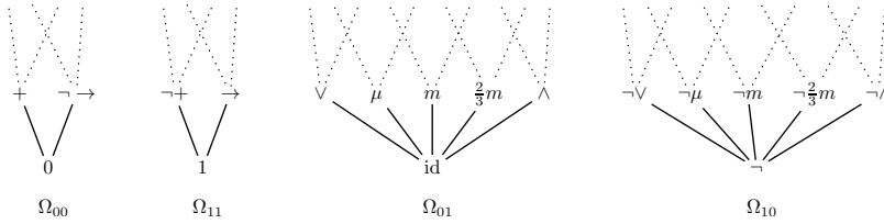
FIGURE 1 The subfunction quasiorder on Boolean functions
