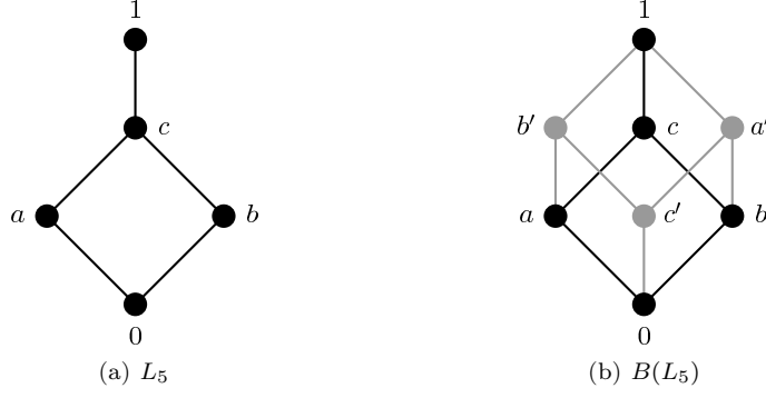
FIGURE 1. A distributive lattice and its Boolean algebra
