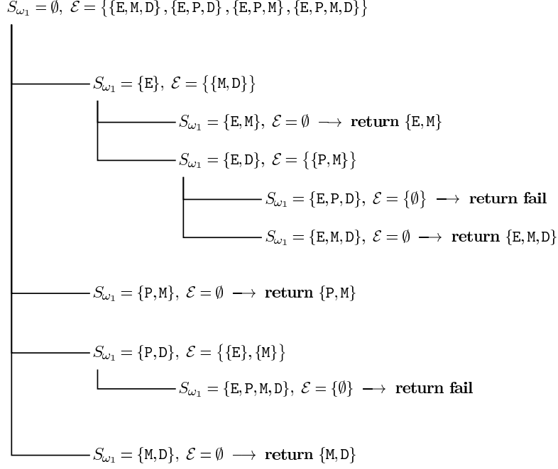
FIGURE 2. Computing S_{\omega_1}
