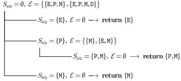
FIGURE 3. Computing S_{\omega_2}
