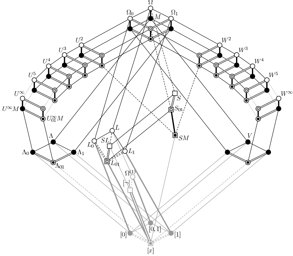
FIGURE 3. The Post lattice.
