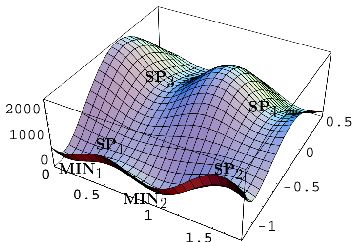
Fig. 1. 2D model potential energy surface.
