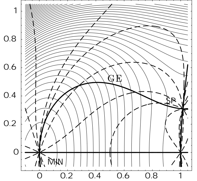
Fig. 9. RGF (dotted lines) and GE on model {4}.
