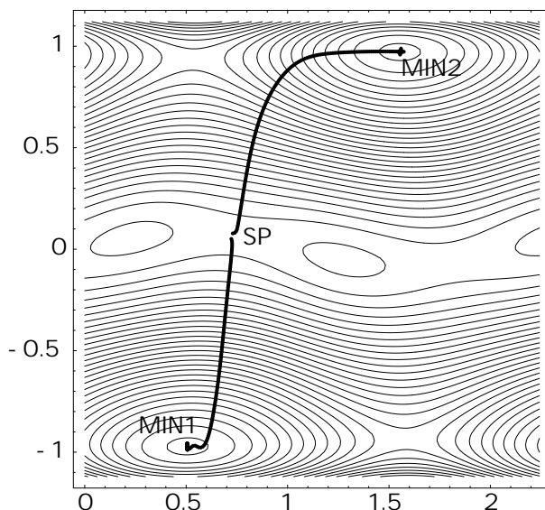
Fig. 4. IRC on test surface \{2\} .
