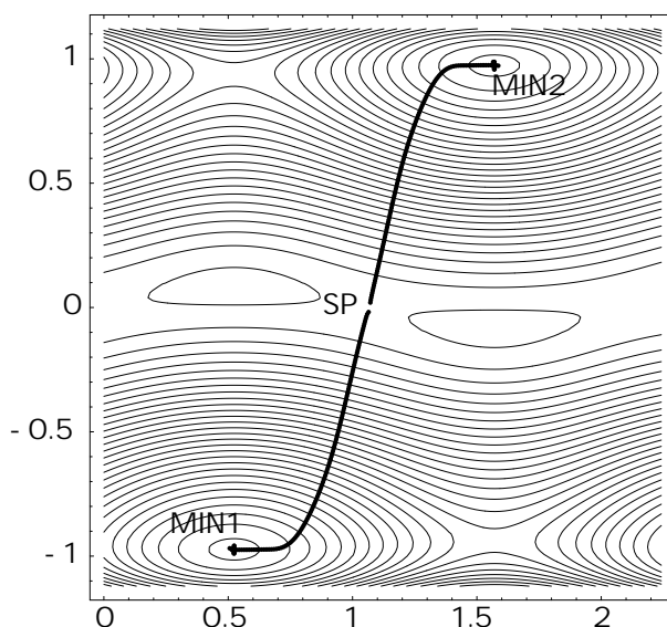
Fig. 2. IRC on test surface \{1\} 51 .
