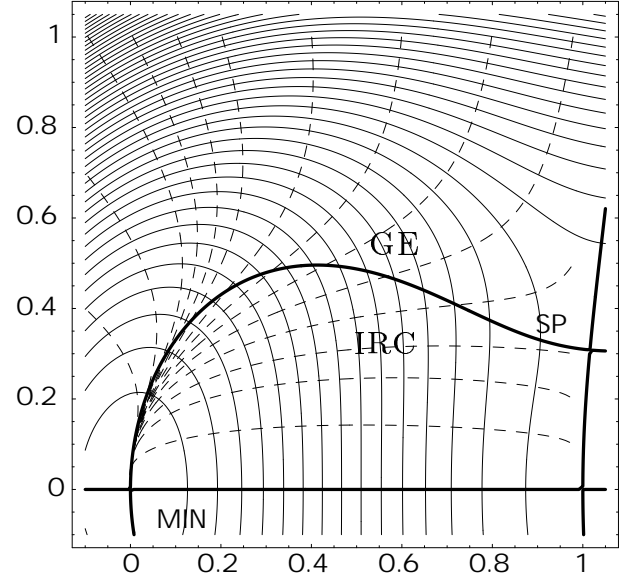
Fig. 14. PES of sample \{4\}^{96} with GE. Steepest descent paths cross the GE, or confluent to it.
