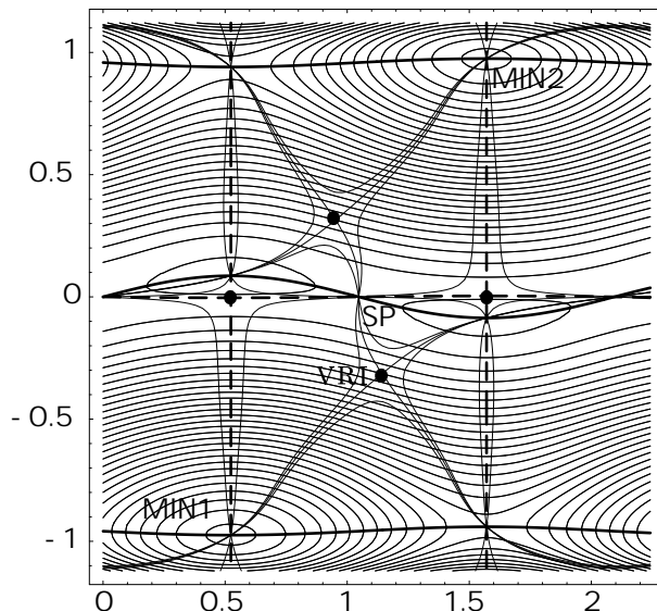
Fig. 7. RGF for PES \{1\}^{51} with VRI points ( \bullet ).
