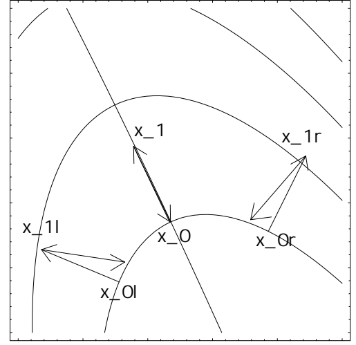
Fig. 12. Scheme of gradient vectors on and near the valley floor. -\mathbf{g}(\mathbf{x}_{1l}) and -\mathbf{g}(\mathbf{x}_{1r}) are used for corrector steps.
