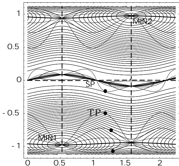
Fig. 5. RGF curves for the torsional transition on surface {1} with turning points (•).
