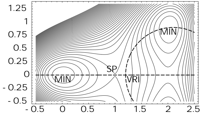
Fig. 11. RGF (dotted curve) bifurcates at the VRI.
