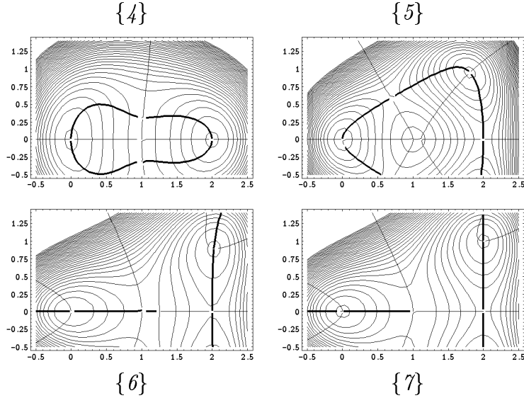
Fig. 10. Examples with valley GEs (bold faced curves).
