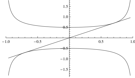
Figure 3.1: Estimating the deviation
