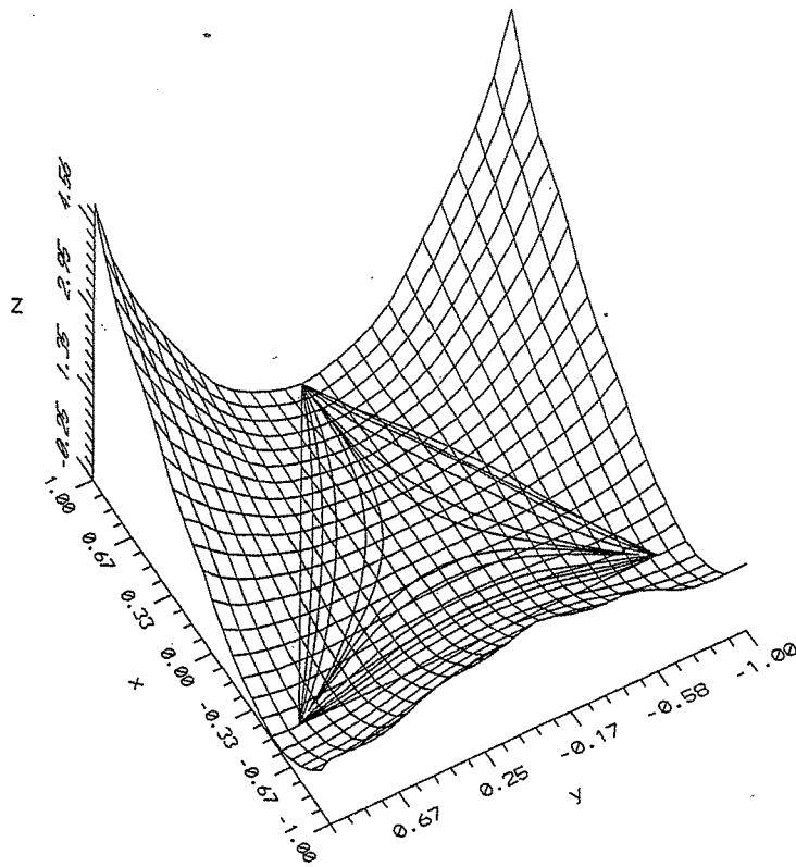
Fig. 6. Phase curves C^t of fig. 5 embedded in the PES of U_M .
