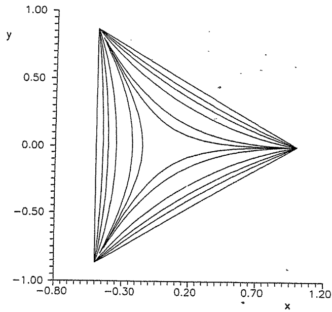
Fig. 5. Phase curves C^t in the plane, calculated by the conventional DDRP method, up to the virtual time t = 350 .
