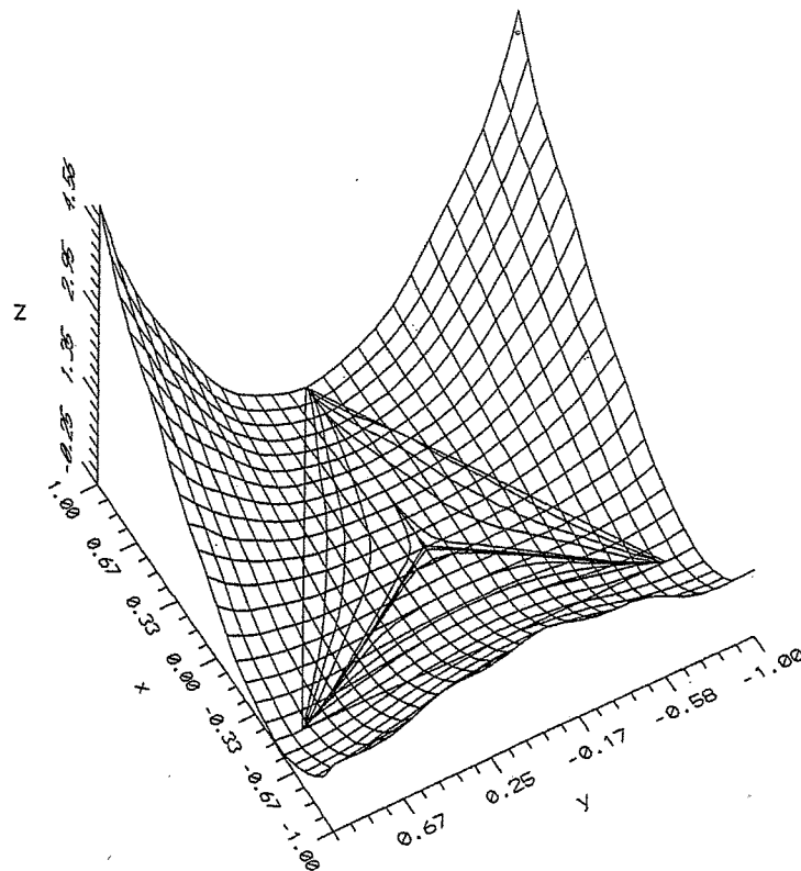
Fig. 8. Phase curves K^t of fig. 7 embedded in the PES of U_M .
