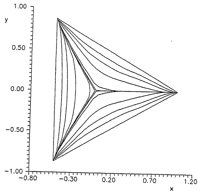
Fig. 7. Phase curves K^t in the plane, calculated by a square-root modified DDRP method, up to the same virtual time t = 350 as in fig. 5.
