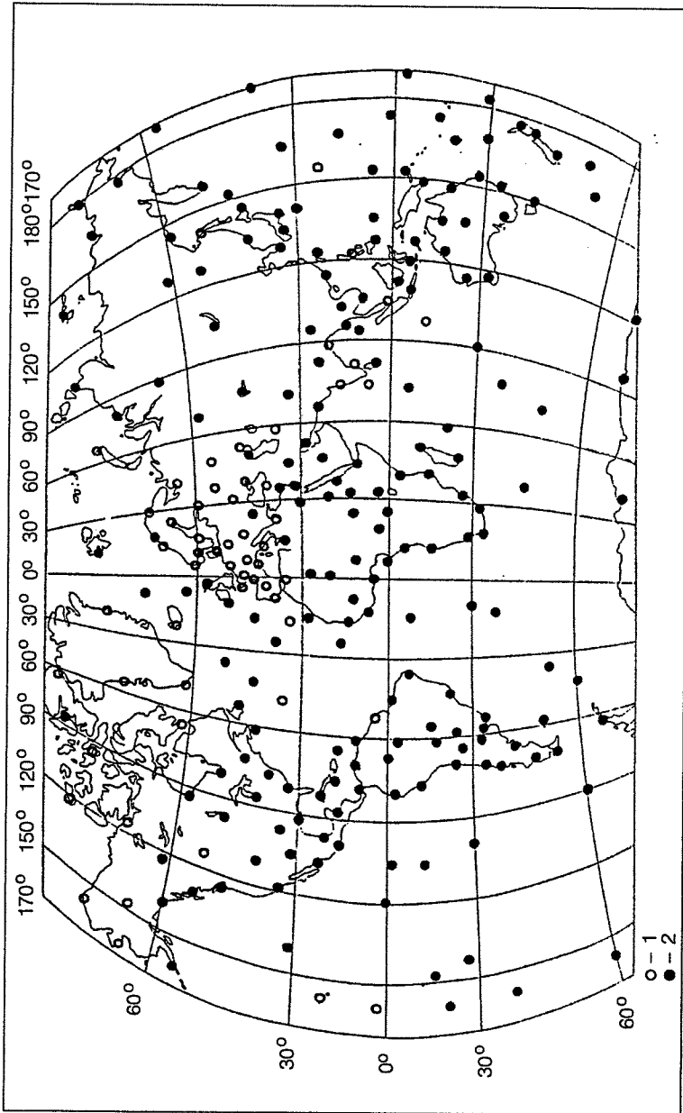
Fig. 5. Stations reconstructing the original pressure field with 85% accuracy, January. Explanations as in Fig. 2
