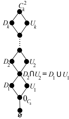
Fig. 4 The lattice of binary invariant relations of \mathcal{C}_k
