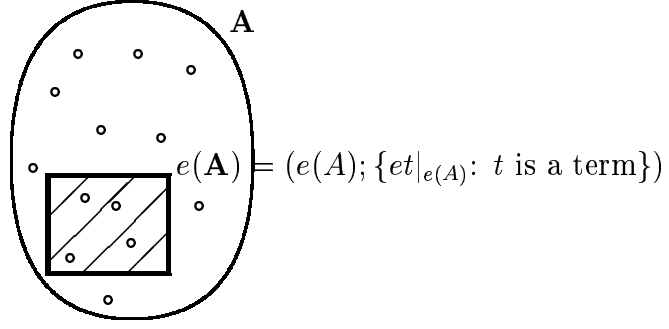
Figure 1: Construction of e(\mathbf{A})
