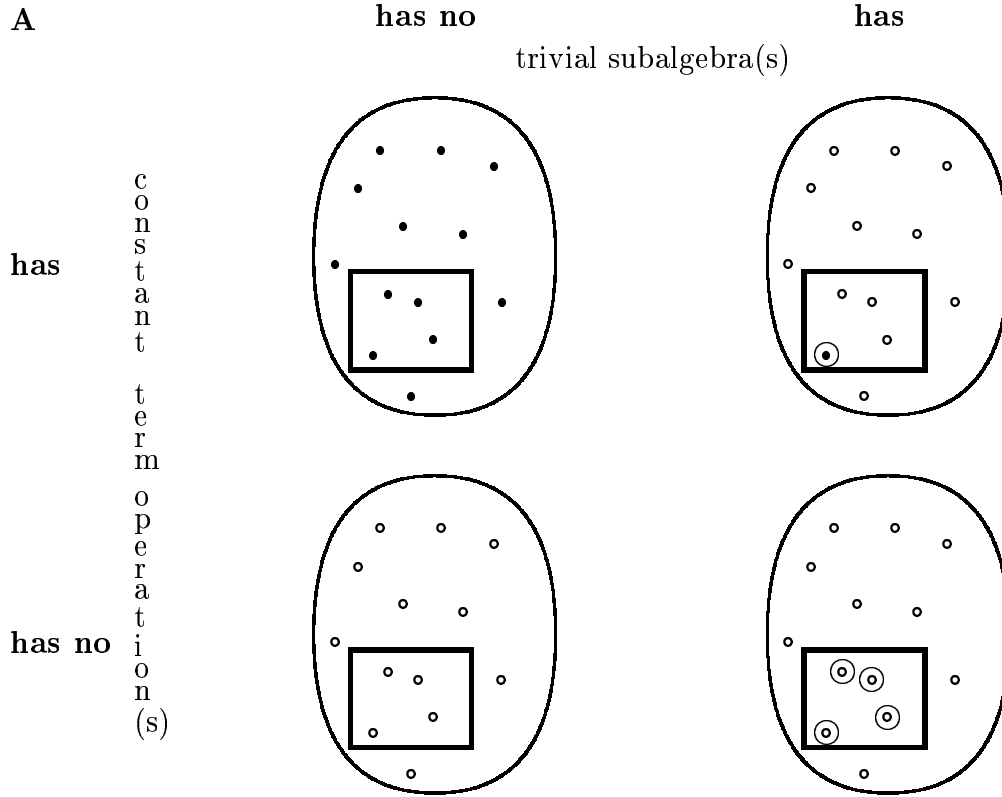
Figure 2: The four classes of strictly simple algebras
